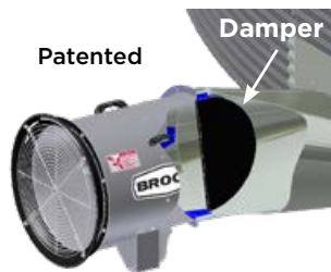
Patented Axial fan butterfly back-draft damper cutaway view with damper open
