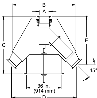
45° FLAT BACK DISTRIBUTOR
