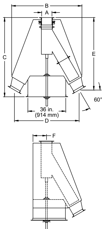
60° FLAT BACK DISTRIBUTOR
